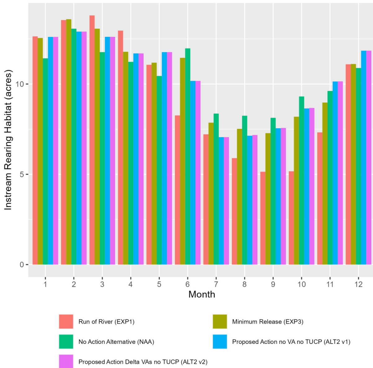
Figure 4-30). Reductions in instream rearing habitat availability in July through October correspond to months of reduced flow. Increased mean floodplain rearing availability in December through April corresponds with months of elevated winter and spring flows.
